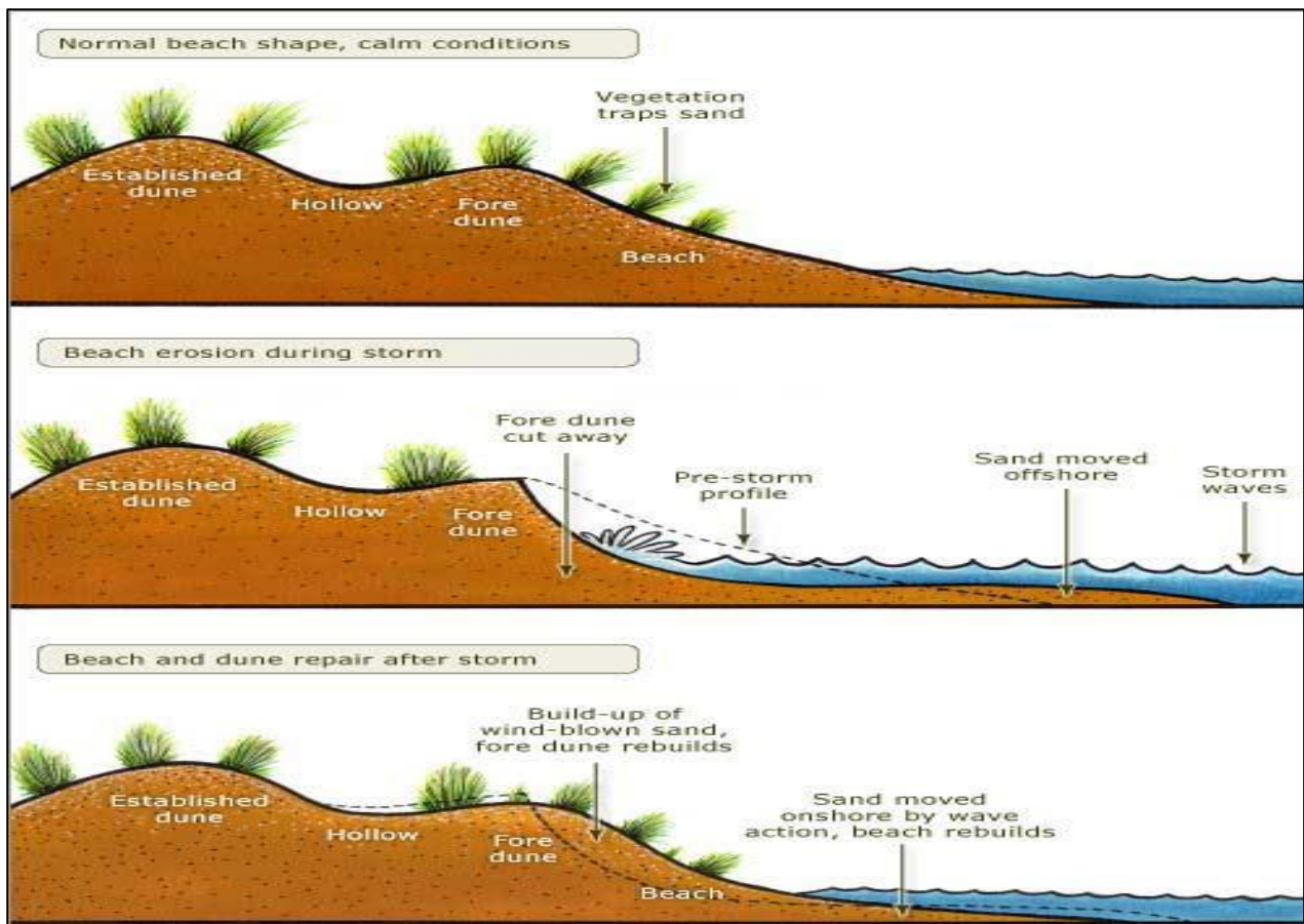
Figure 1: Beach and foredune profiles.
